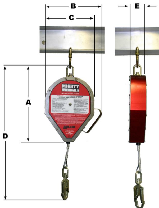
RL50G/50FT shown Dimensions specified on page 2
